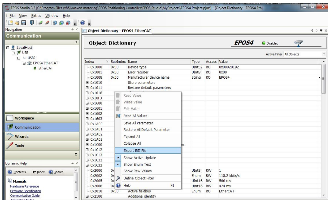
Figure 6-47 EtherCAT integration – Beckhoff TwinCAT | Export ESI file
