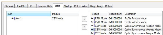
Figure 6-71 EtherCAT integration – Beckhoff TwinCAT | Set CSV settings
