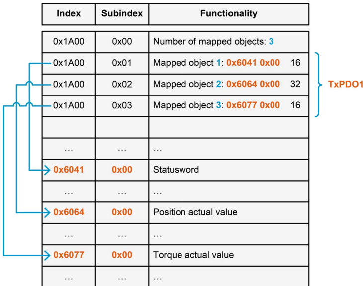
Figure 5-42 CANopen basic information | PDO mapping example
