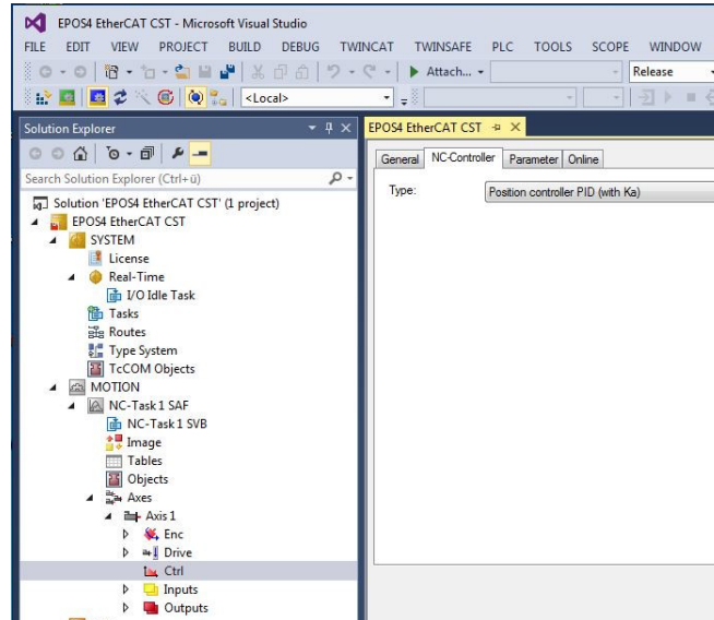
Figure 6-77 EtherCAT integration – Beckhoff TwinCAT | Configure position control type
