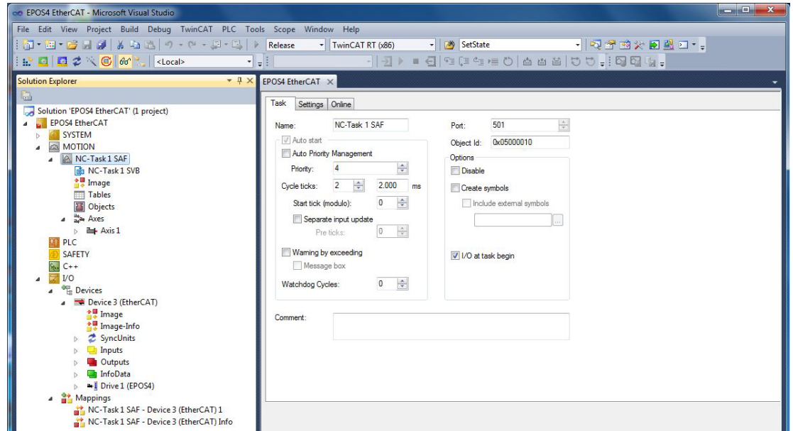
Figure 6-63 EtherCAT integration – Beckhoff TwinCAT | Set cycle ticks 1
