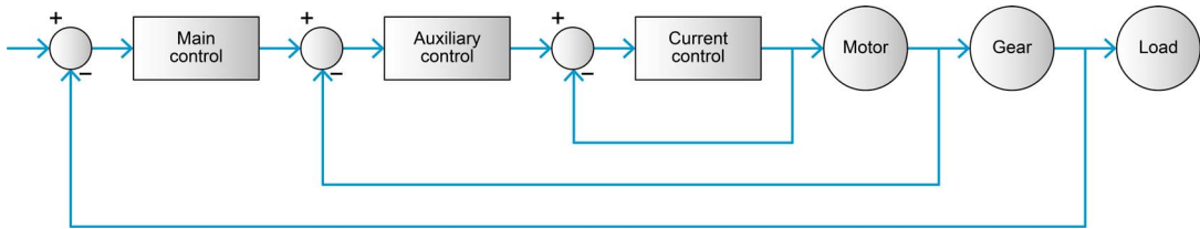
Figure 10-102 Dual loop control | Control structure
