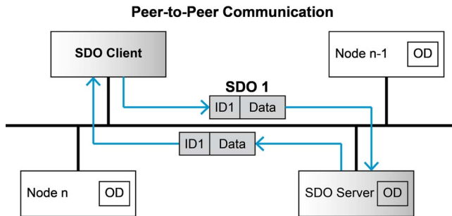
Figure 5-32 CANopen basic information | SDO communication
