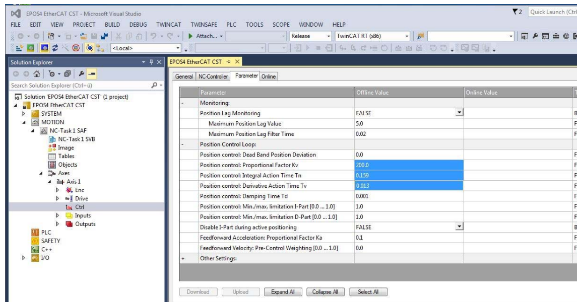
Figure 6-78 EtherCAT integration – Beckhoff TwinCAT | Configure position control parameters
