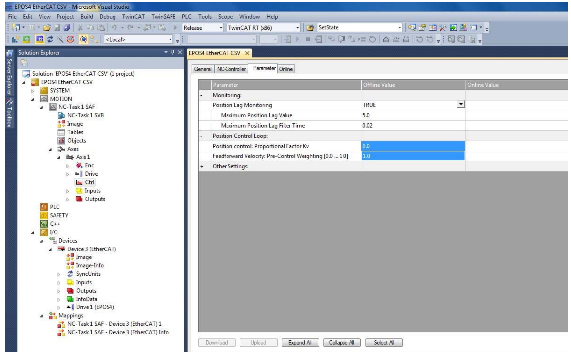
Figure 6-72 EtherCAT integration – Beckhoff TwinCAT | Set position control loop settings
