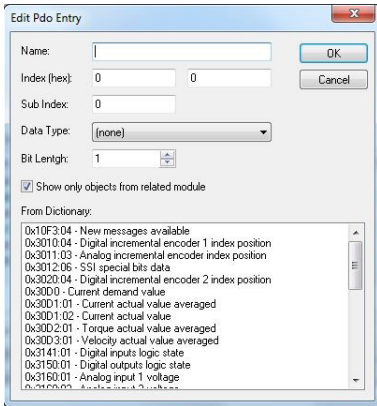
Figure 6-61 EtherCAT integration – Beckhoff TwinCAT | Edit PDO values
