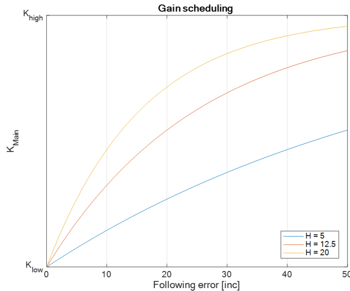
Figure 10-104 Dual loop control | Gain scheduling function for different values of main loop gain scheduling weight
