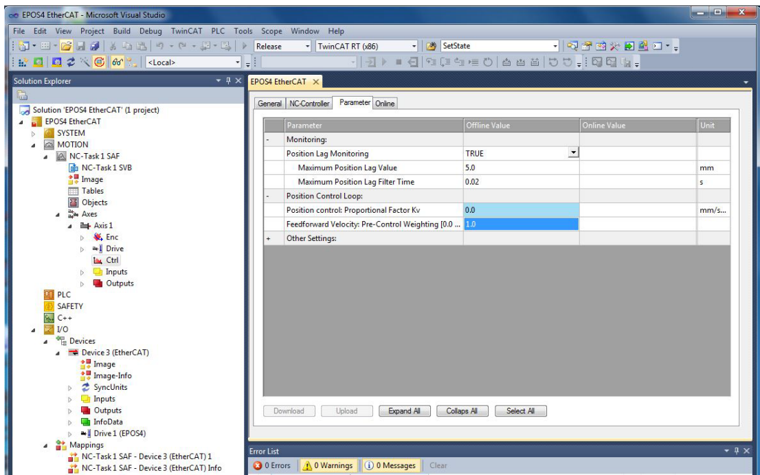
Figure 6-70 EtherCAT integration – Beckhoff TwinCAT | Set position control loop settings
