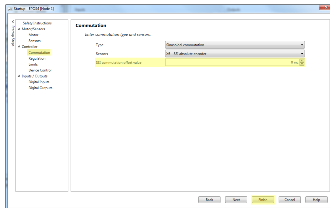
Figure 8-94 Adjustment of SSI commutation offset value | Set SSI commutation offset value
