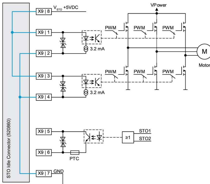
Figure 9-98 Safe Torque Off (STO) | STO Idle Connector
