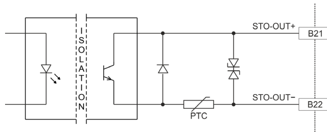
Figure 9-101 Safe Torque Off (STO) | STO-OUT circuit
