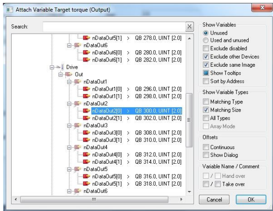
Figure 6-76 EtherCAT integration – Beckhoff TwinCAT | Configure position control loop
