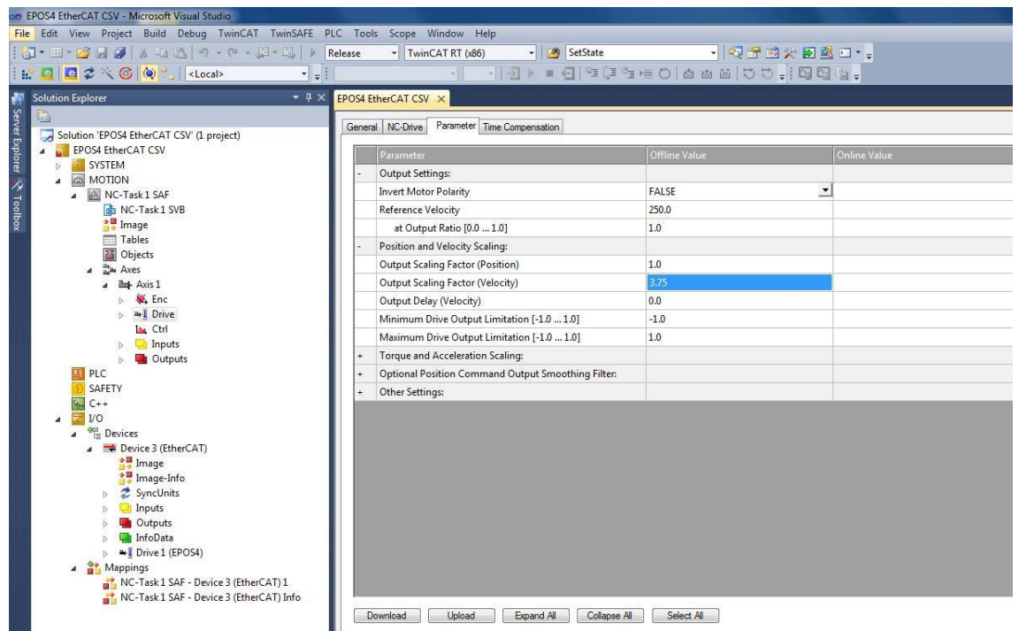
Figure 6-73 EtherCAT integration – Beckhoff TwinCAT | Set output scaling factor
