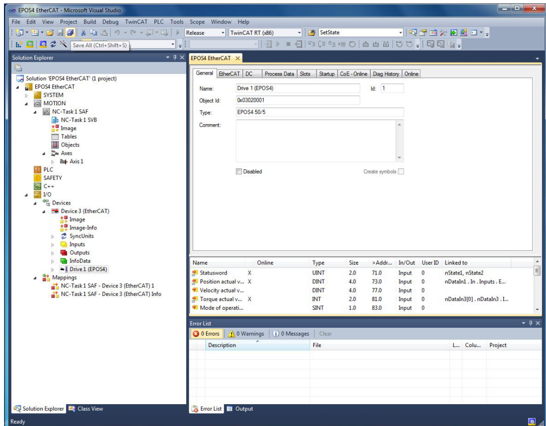
Figure 6-57 EtherCAT integration – Beckhoff TwinCAT | Structure tree
