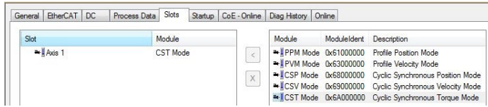
Figure 6-74 EtherCAT integration – Beckhoff TwinCAT | Set CST settings
