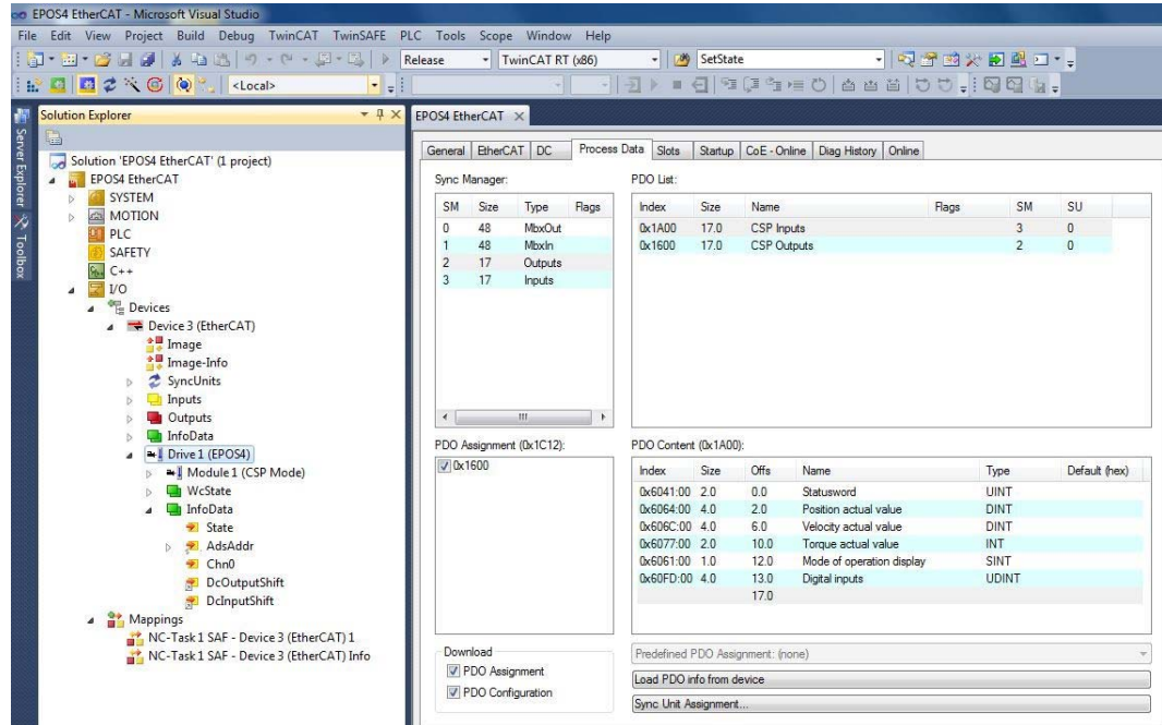
Figure 6-59 EtherCAT integration – Beckhoff TwinCAT | Display process data
