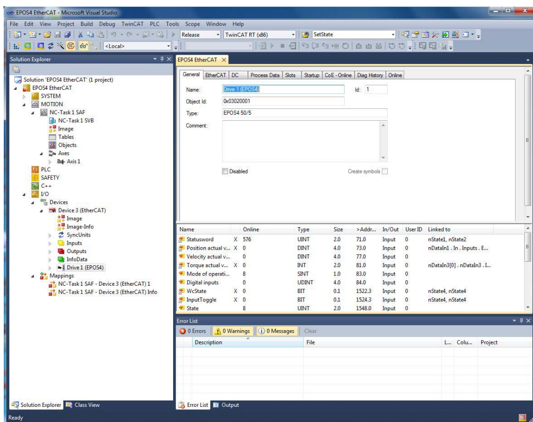
Figure 6-56 EtherCAT integration – Beckhoff TwinCAT | Save project
