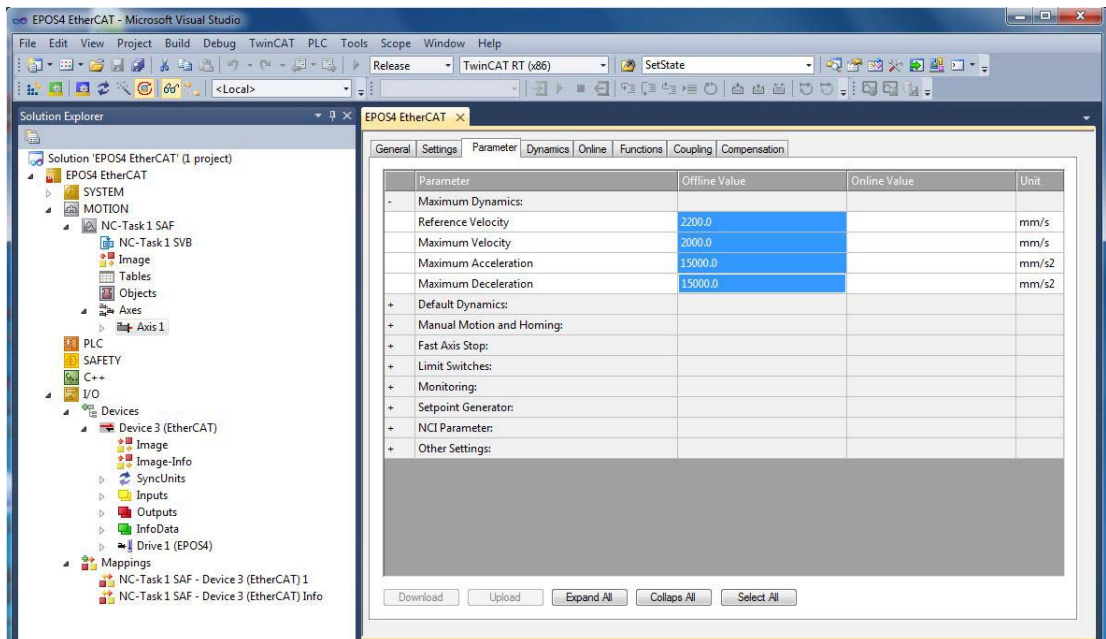
Figure 6-66 EtherCAT integration – Beckhoff TwinCAT | Set speed settings
