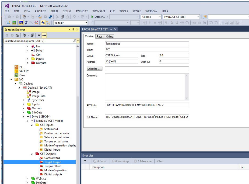
Figure 6-75 EtherCAT integration – Beckhoff TwinCAT | Set target torque
