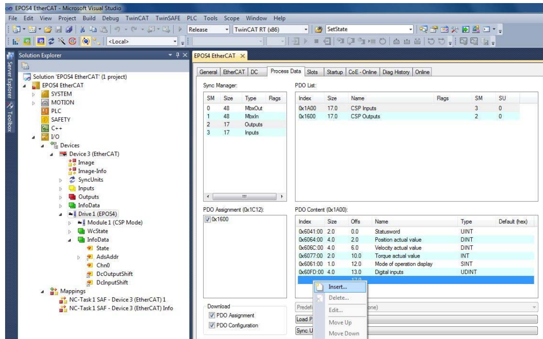
Figure 6-60 EtherCAT integration – Beckhoff TwinCAT | Select PDO
