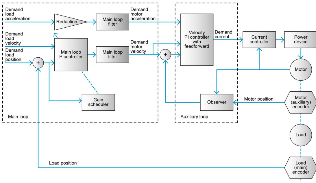
Figure 10-103 Dual loop control | Control structure in detail
