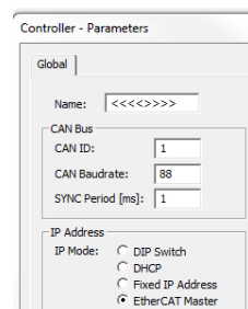
Figure 6-82 EtherCAT integration – zub's MACS Multi-Axis EtherCAT Masters | MACS5 IP Mode Configuration
