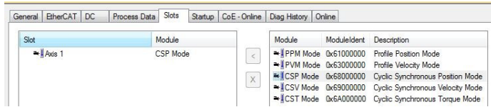
Figure 6-69 EtherCAT integration – Beckhoff TwinCAT | Set CSP settings
