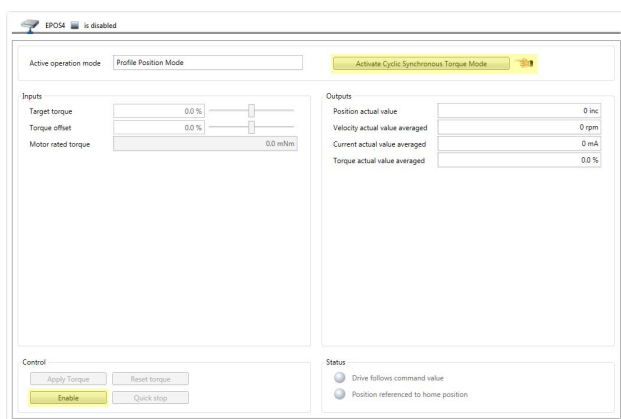
Figure 8-89 Adjustment of SSI commutation offset value | Activate CST
