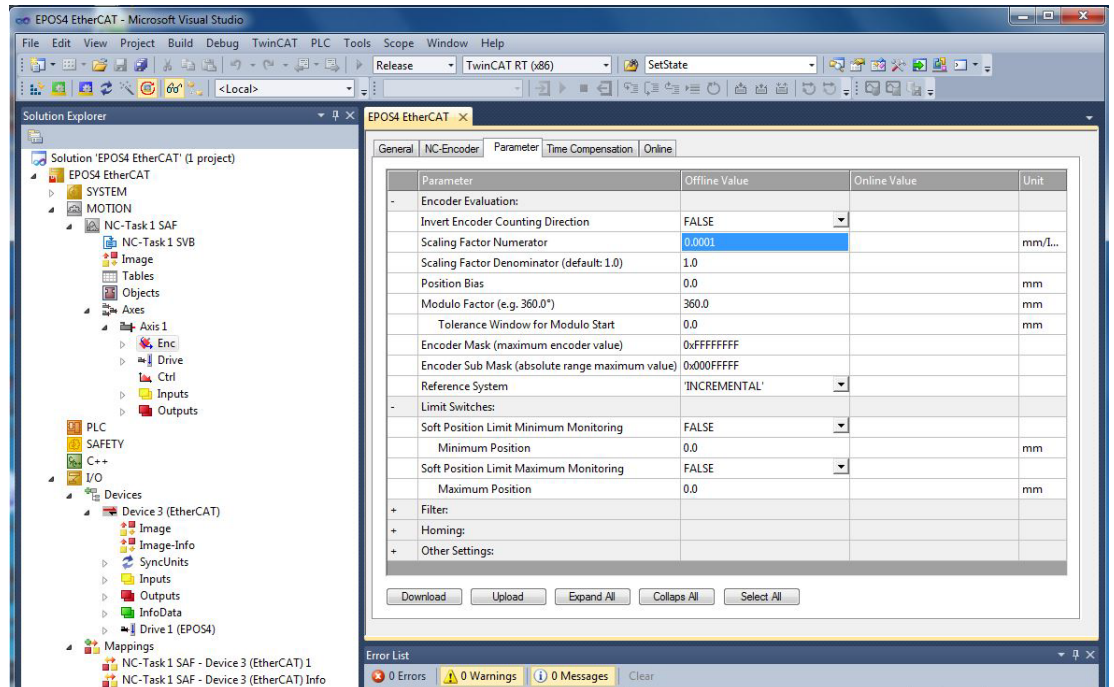
Figure 6-68 EtherCAT integration – Beckhoff TwinCAT | Set encoder settings
