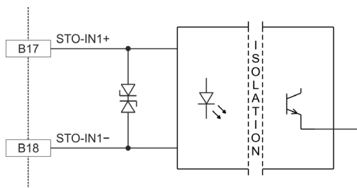
Figure 9-99 Safe Torque Off (STO) | STO-IN1 circuit (analogously valid for STO-IN2)
