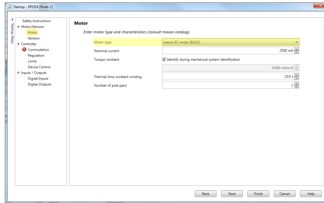
Figure 8-93 Adjustment of SSI commutation offset value | Select motor type maxon EC motor
