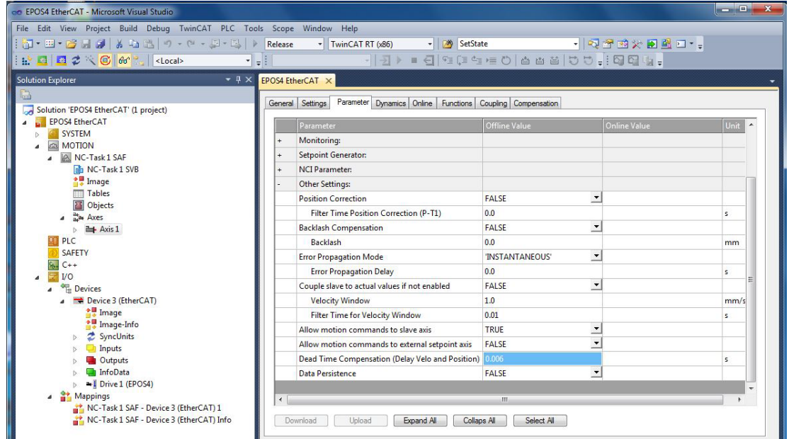
Figure 6-67 EtherCAT integration – Beckhoff TwinCAT | Set dead time compensation
