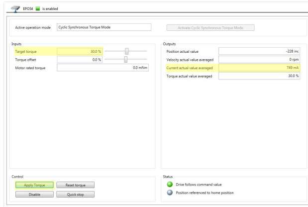
Figure 8-90 Adjustment of SSI commutation offset value | Apply target torque
