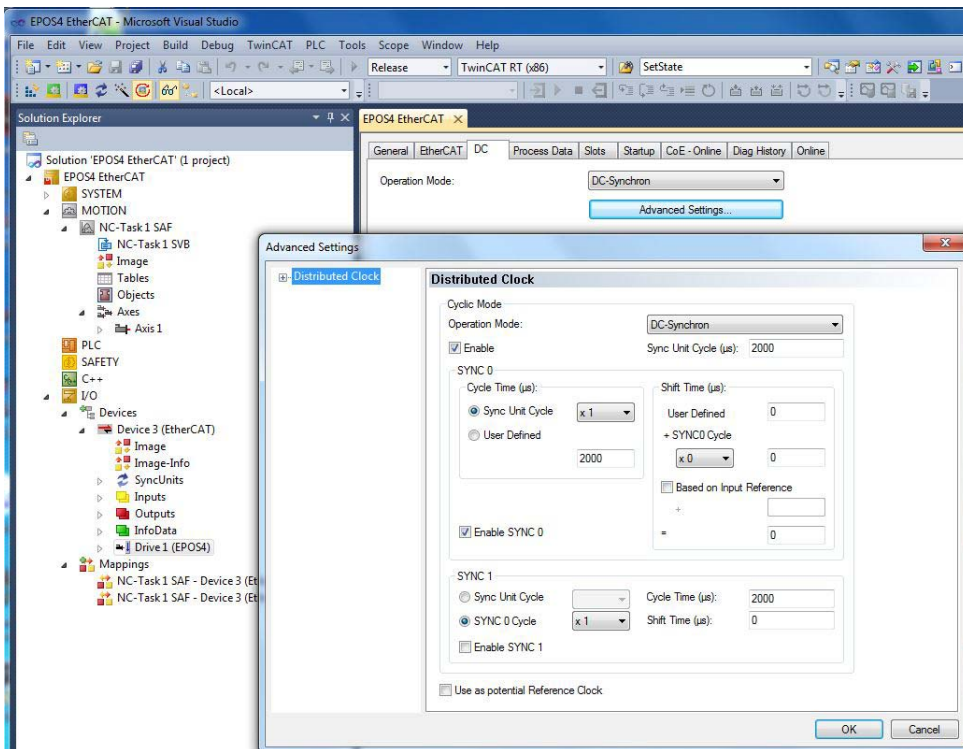
Figure 6-62 EtherCAT integration – Beckhoff TwinCAT | Set distributed clock
