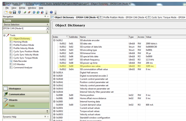
Figure 8-91 Adjustment of SSI commutation offset value | Read SSI position raw value
