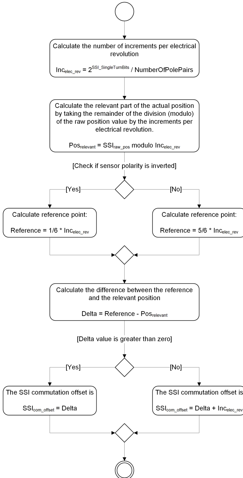
Figure 8-92 Adjustment of SSI commutation offset value | Determine SSI commutation offset value
