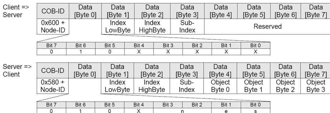
Figure 5-33 CANopen basic information | SDO upload protocol (expedited transfer) – Read
