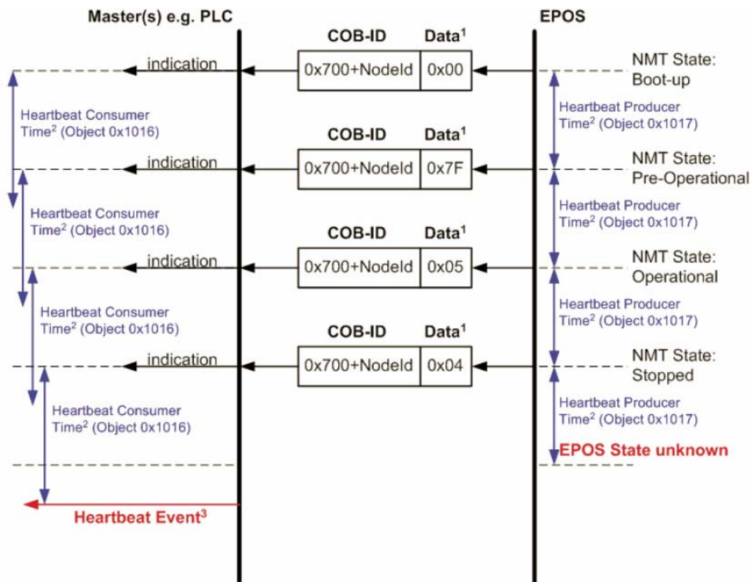
Figure 5-46 CANopen basic information | Heartbeat protocol – Timing diagram
