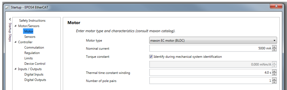
Figure 6-79 EtherCAT integration – zub's MACS Multi-Axis EtherCAT Masters | EPOS Studio "Startup Wizard"
