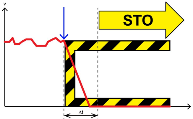
Figure 9-96 Safe Torque Off (STO) | Working principle
