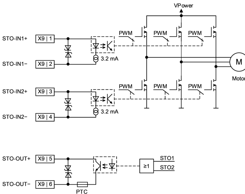
Figure 9-97 Safe Torque Off (STO) | Functional diagram
