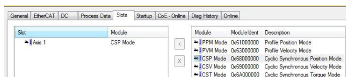
Figure 6-58 EtherCAT integration – Beckhoff TwinCAT | Configure slots
