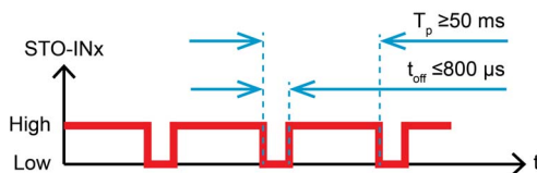
Figure 9-100 Safe Torque Off (STO) | Test pulses
