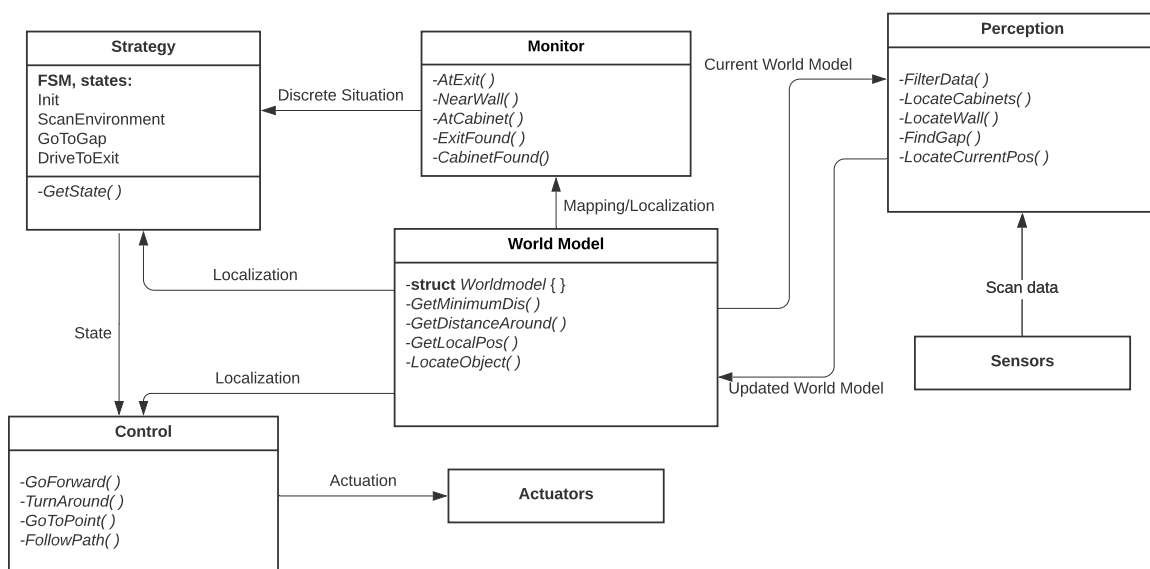
Figure 1: Information architecture of the system.
